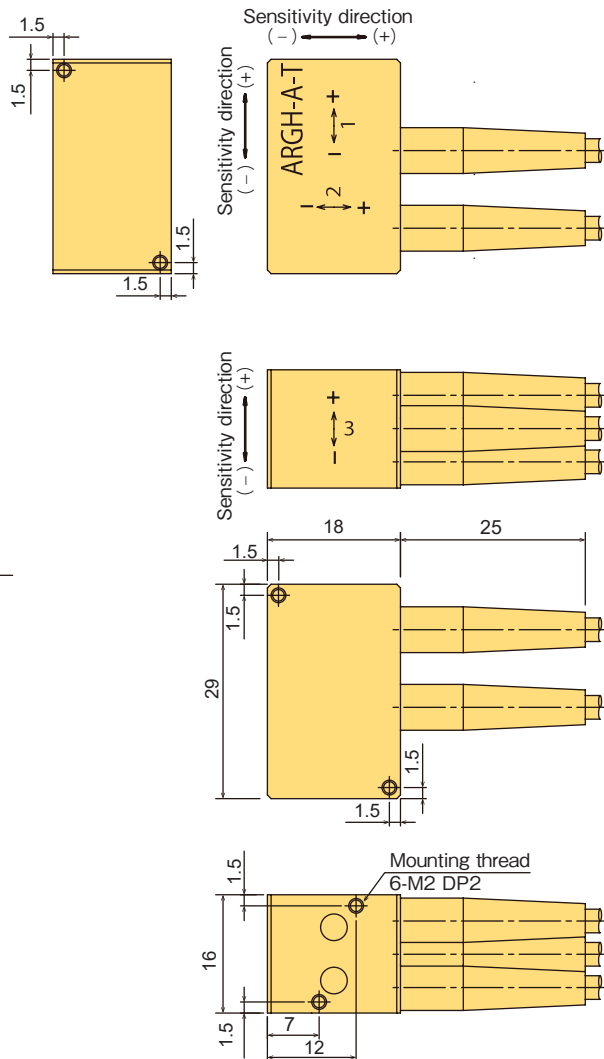
Acceleration transducer
