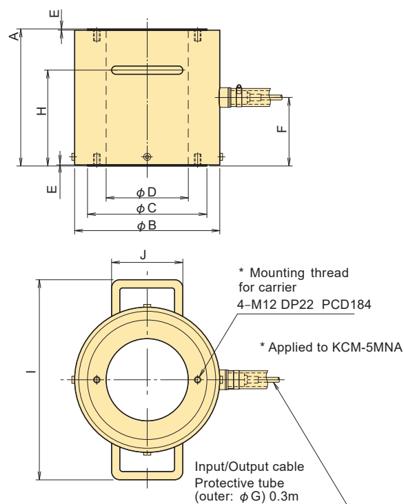
KCM-2MNA~ 5MNA
