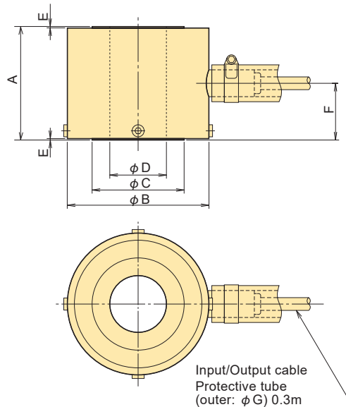
KCM-2MNA~ 5MNA
