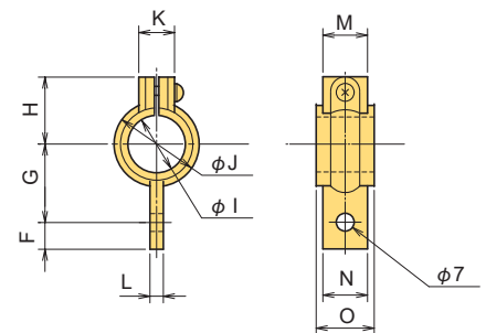
HOLDER CDPF-11
