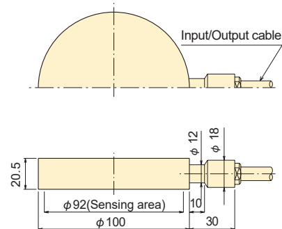
KDC-PA
