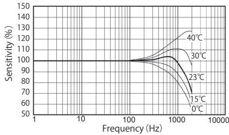
Acceleration transducer presents different frequency characteristics, output sensitivity vs. frequency, depending on temperature.
