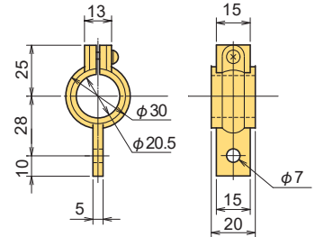
HOLDER CDPF-11-25
