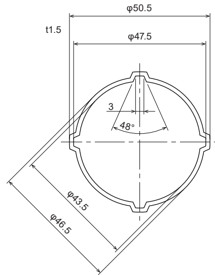
\Phi 50\text{mm} Roller for Guide Pipes
