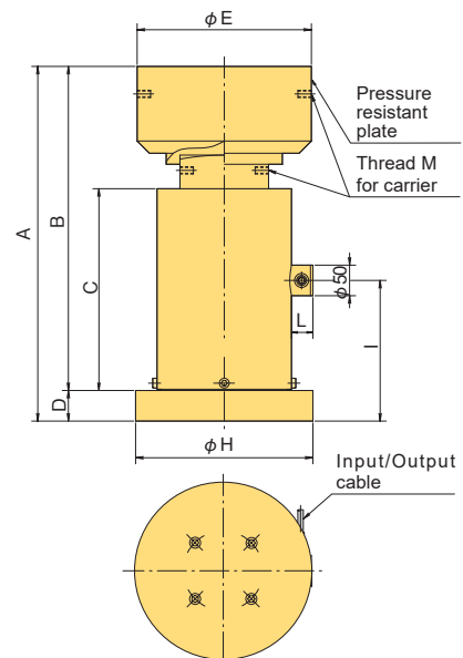
CLJ-5MN, -10MNB
