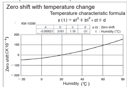
Example of individual temperature data
